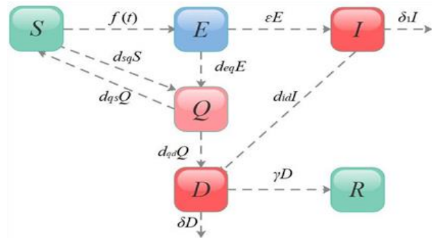
Figure 1: Warehouse transfer diagram of SEIQDR Model
